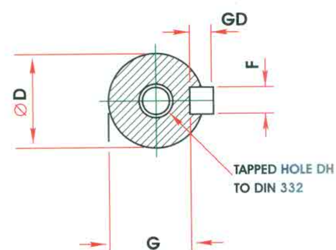
SHAFT DIA
